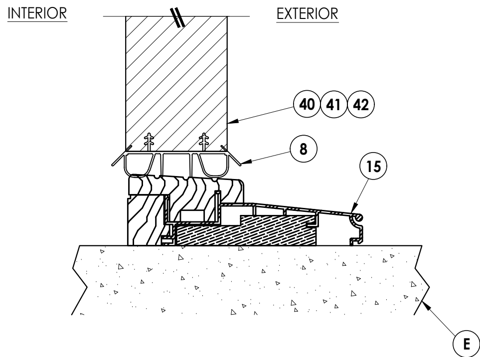
2 9 VERTICAL CROSS SECTION Inswing
