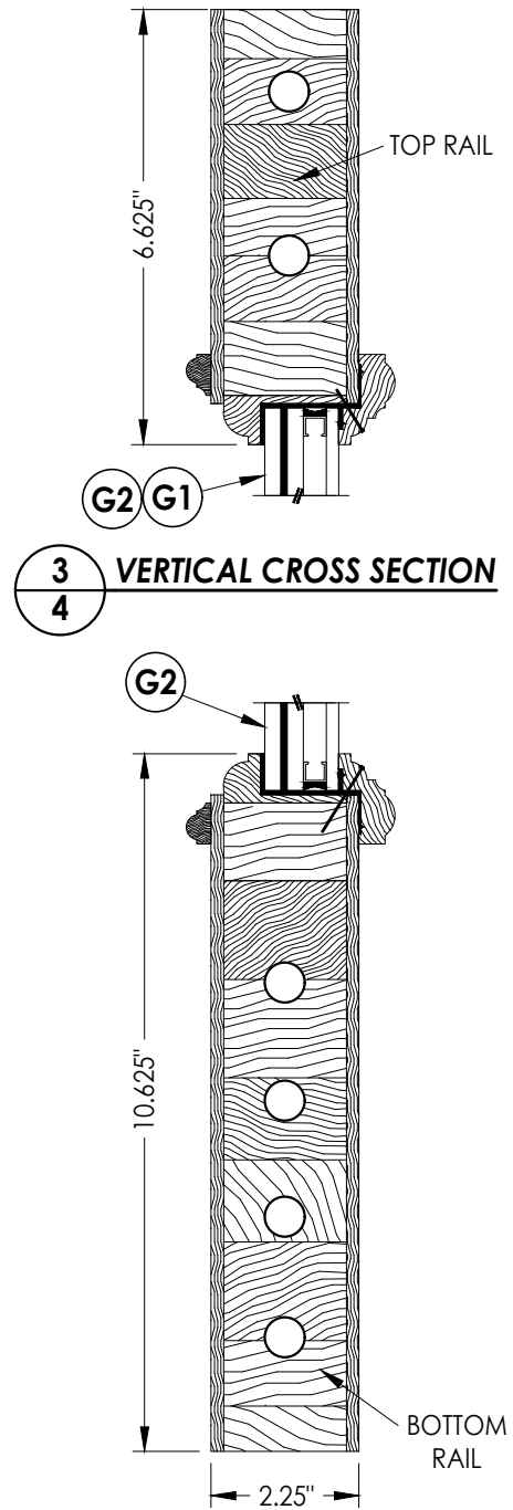
5 VERTICAL CROSS SECTION 4
